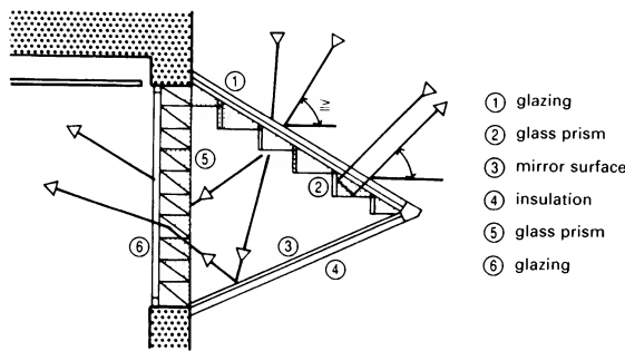
52 Prismatic redirection of light
